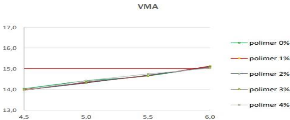
Figure 5. VMA Recapitulation Graph
