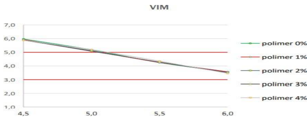
Figure 4. VIM (Voids in Mixture) Recapitulation Graphic
